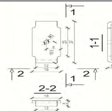
H=16 mm, W=25-37, Screw M3-30
