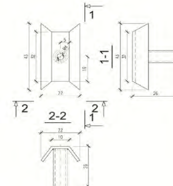
H=22 mm, W= 43mm, Screw M4-30
