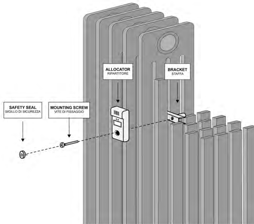
Figure 2. [Left side] How to mount the allocator in a ribs heater using the appropriate mounting brackets. [Right side] How to install the remote sensor version of the allocator.
